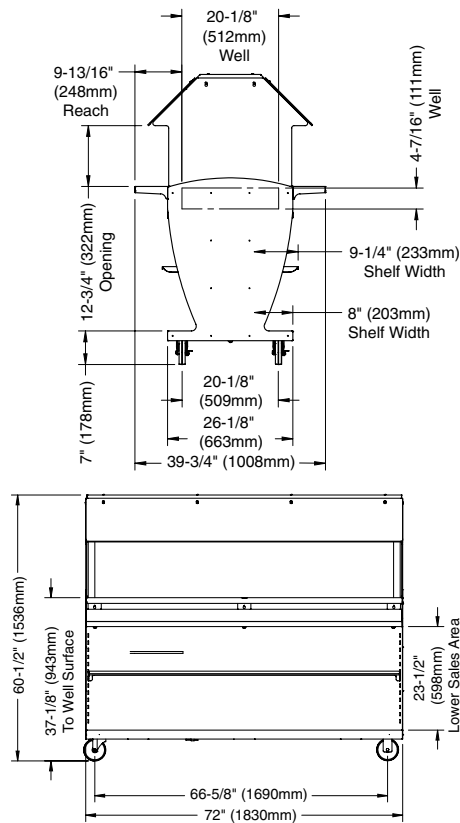
HFT2SYS-500 Standard
